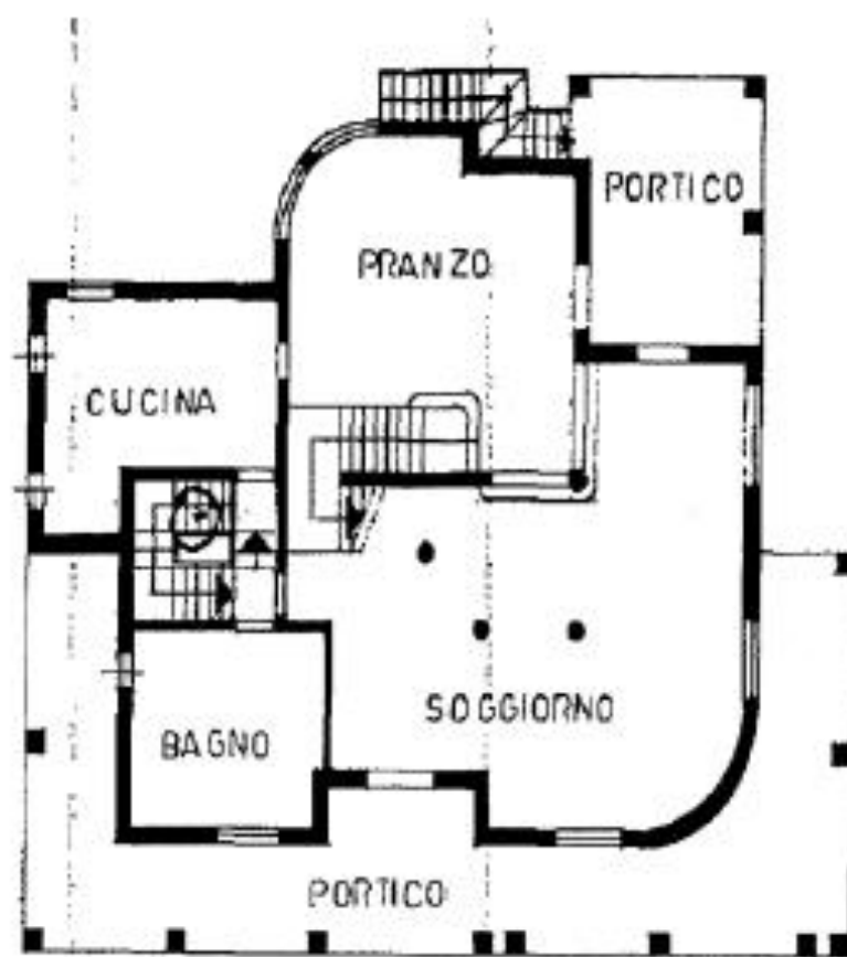
PIANO TERRA H 2,70
